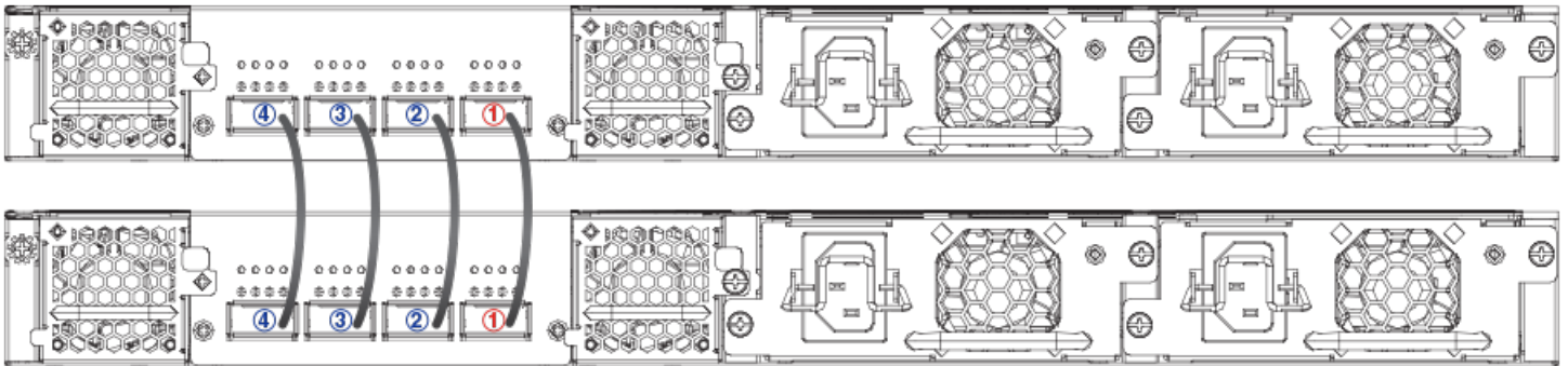
FIGURE 35 ICX 7650-48ZP Two-unit Stack Linear-topology Trunk (100 Gbps)
