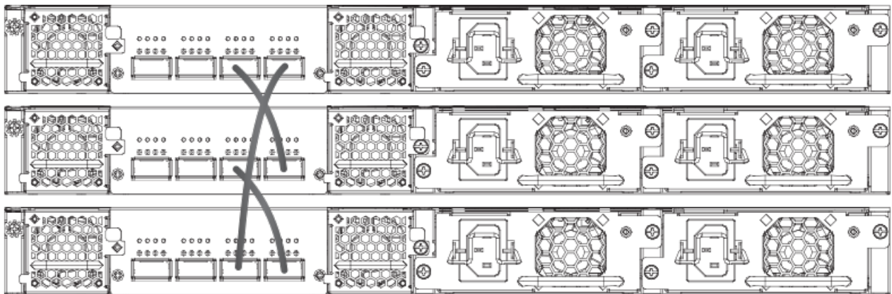
FIGURE 31 ICX 7650 100-Gbps Ring Stack
