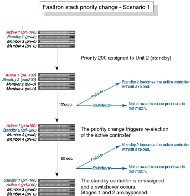
FIGURE 47 Scenario 1 - Hitless Stacking Switchover After a Priority Change
