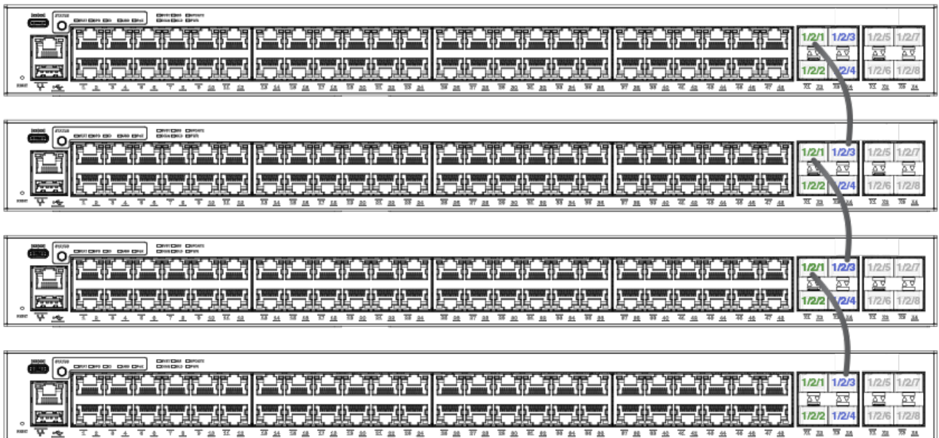
FIGURE 10 ICX 7150-48ZP Linear Stack
