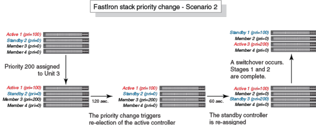
FIGURE 48 Scenario 2 - Hitless Stacking Switchover After a Priority Change
