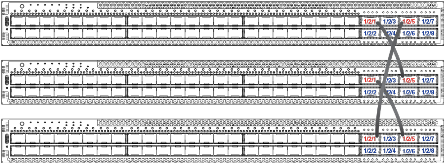
FIGURE 39 ICX 7850-48C/48F/48FS Ring Topology
