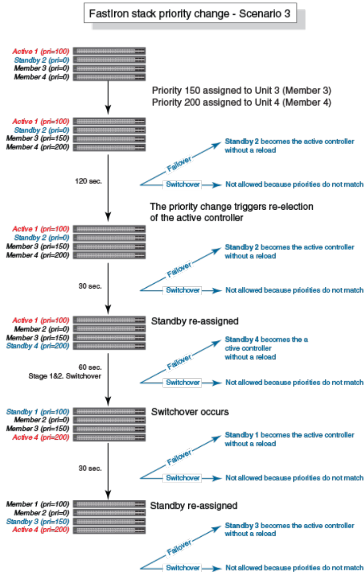
FIGURE 49 Scenario 3 - Hitless Stacking Switchover After a Priority Change
