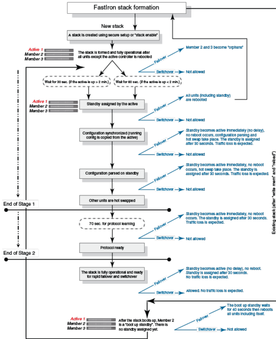
FIGURE 41 Hitless Stacking Support During Stack Formation
