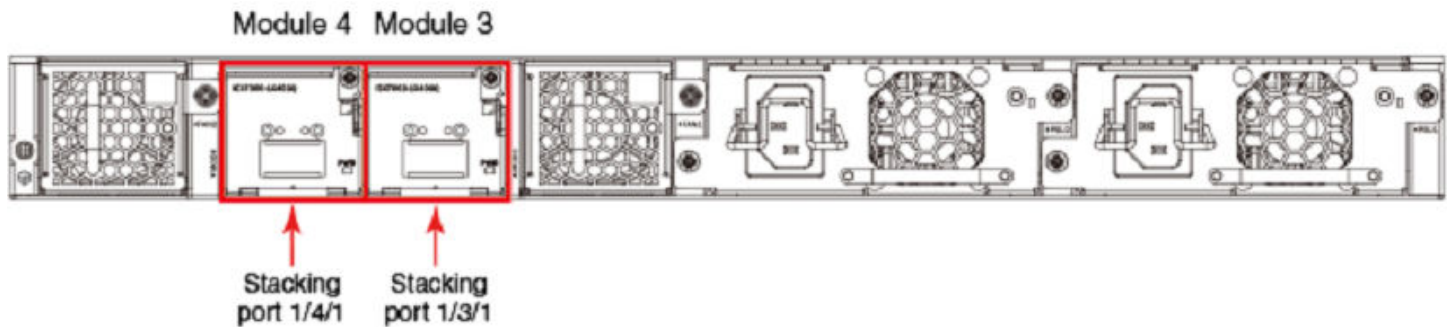
FIGURE 17 ICX 7450 1 X 40-Gbps Valid-stack-ports
