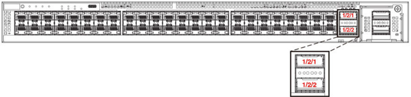
FIGURE 25 ICX 7550 Stacking Ports
