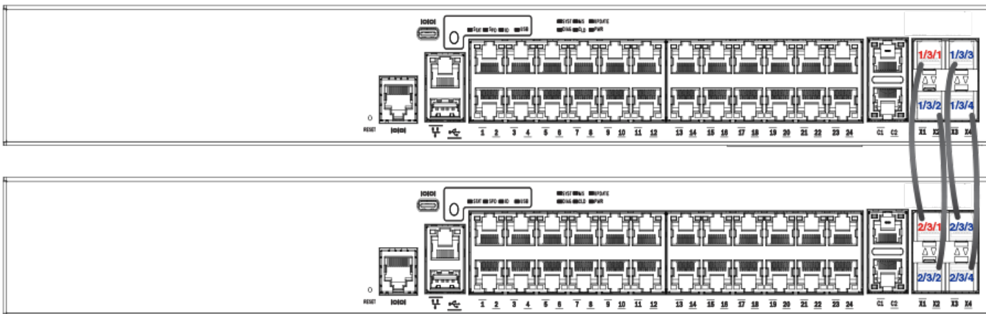
FIGURE 12 ICX 7150 24-port Two-unit Stack with Linear-topology Trunk
