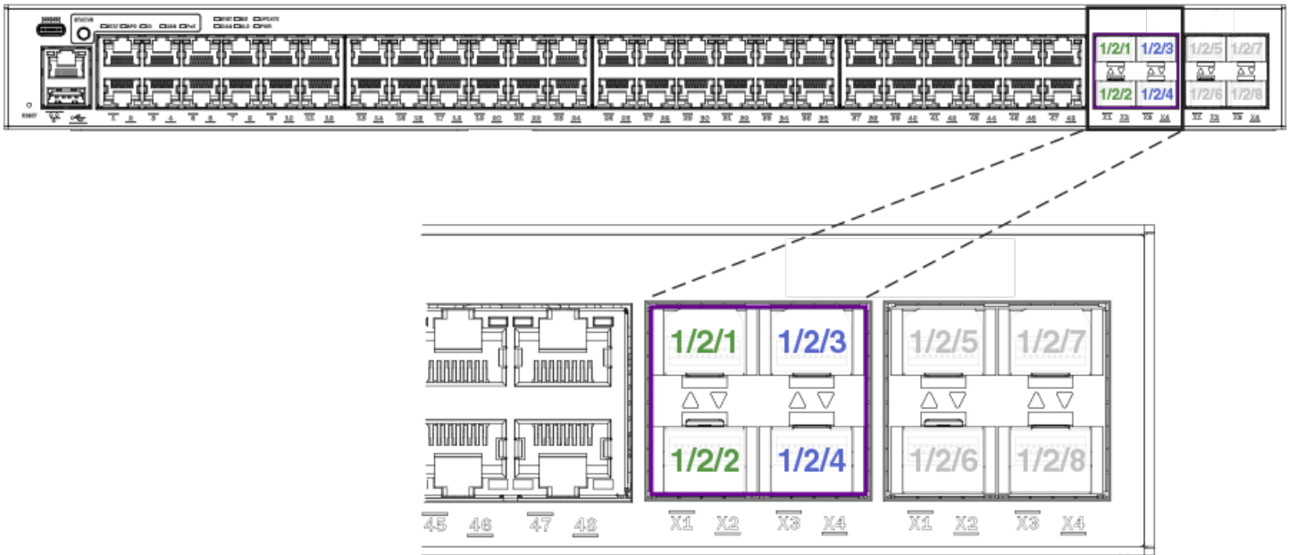
FIGURE 5 ICX 7150-48ZP Stacking Ports
