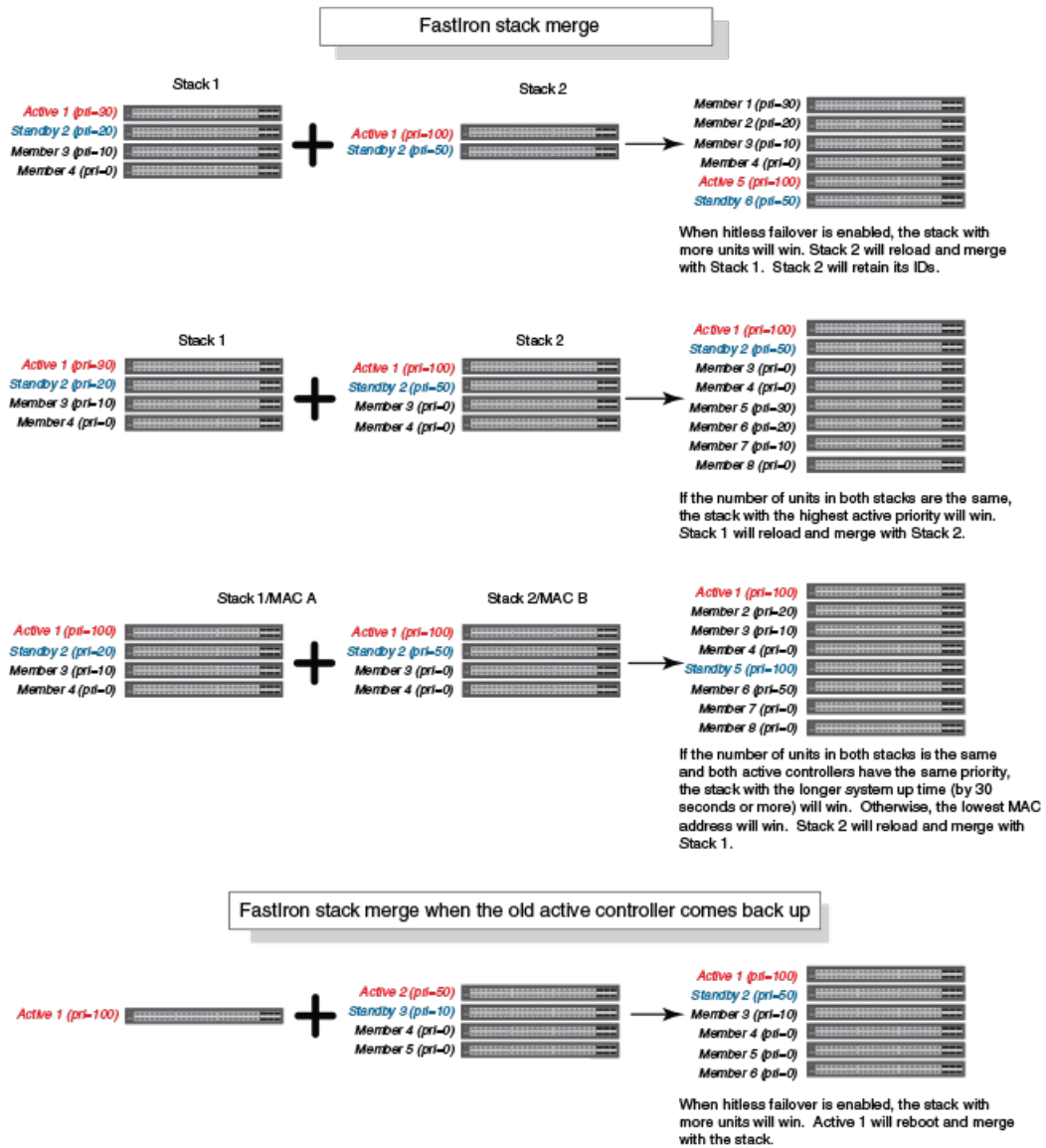
FIGURE 42 Hitless Stacking Support During a Stack Merge
