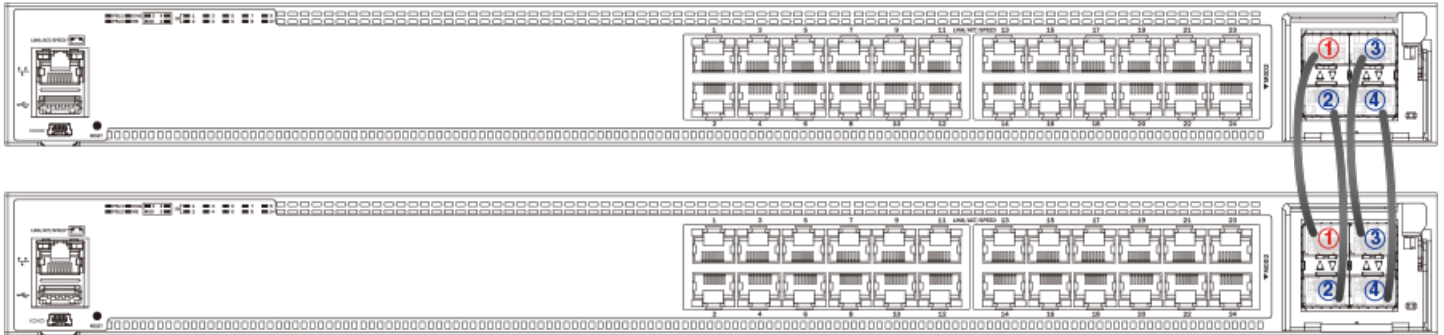
FIGURE 24 ICX 7450-24P Two-unit Stack with Linear-topology Trunk (Rear Panel)
