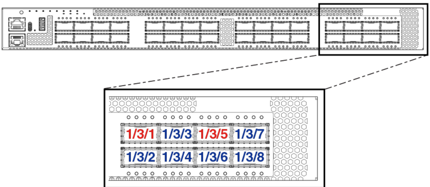
FIGURE 36 ICX 7850-32Q Stacking Ports
