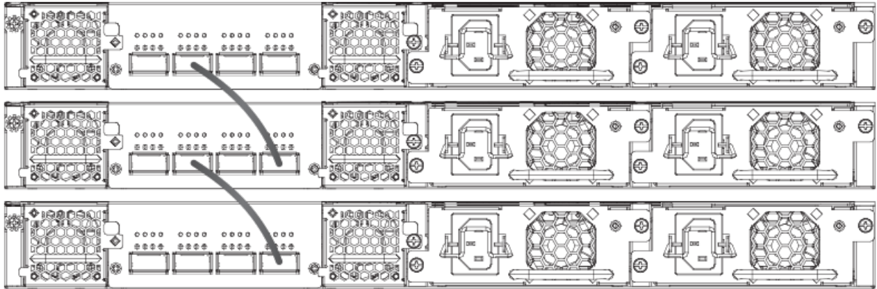
FIGURE 32 ICX 7650 40-Gbps Linear Stack
