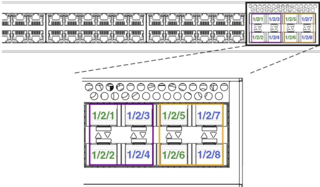
FIGURE 13 ICX 7250 Stacking Ports
