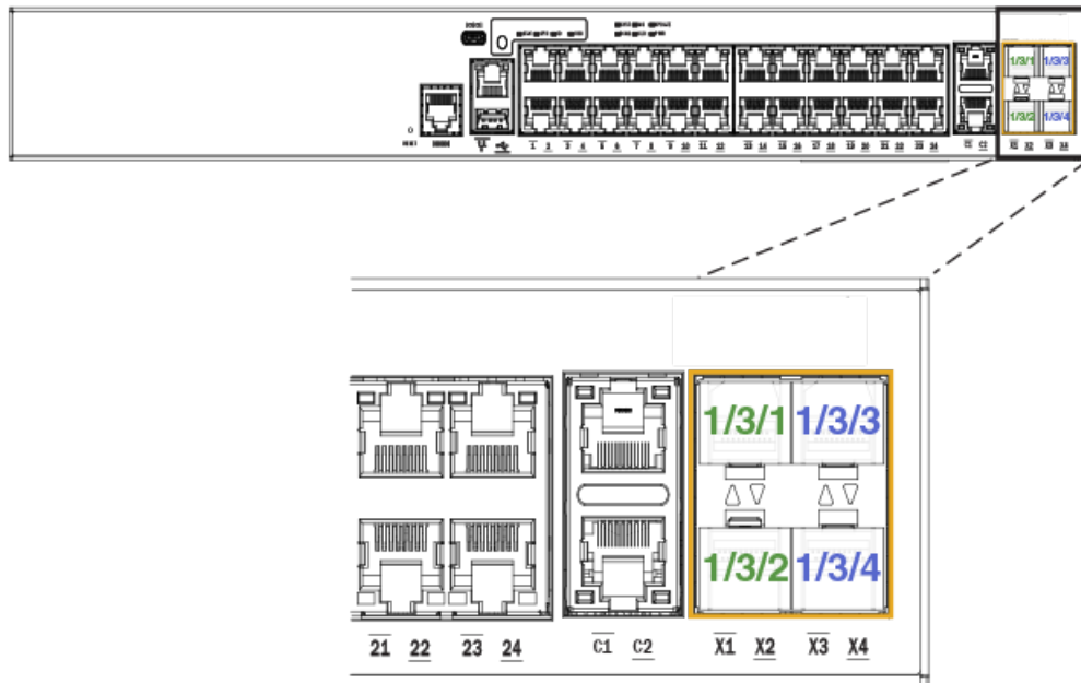
FIGURE 4 ICX 7150 Stacking Port Location on 24-port and Some 48-port Models
