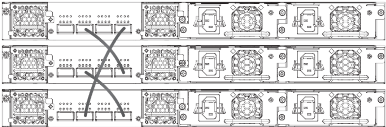
FIGURE 33 ICX 7650 40-Gbps Ring Stack
