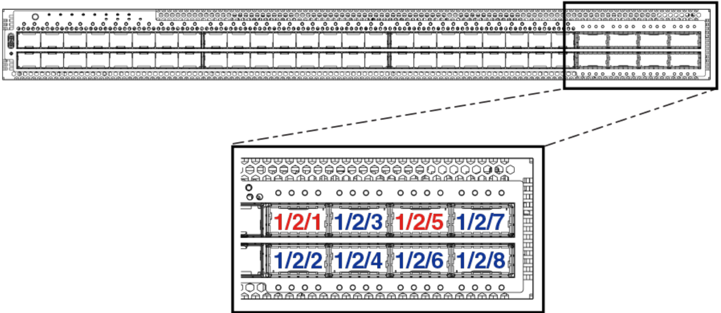
FIGURE 37 ICX 7850-48C/48F/48FS Stacking Ports
