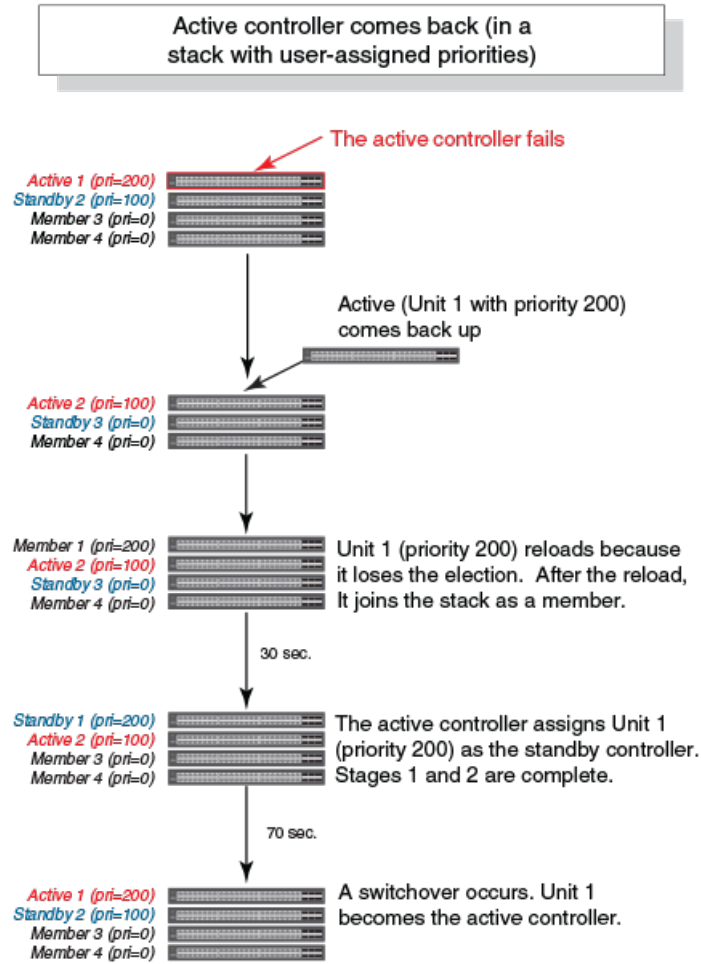
FIGURE 46 Hitless Stacking Switchover When the Active Controller Comes Back Up
