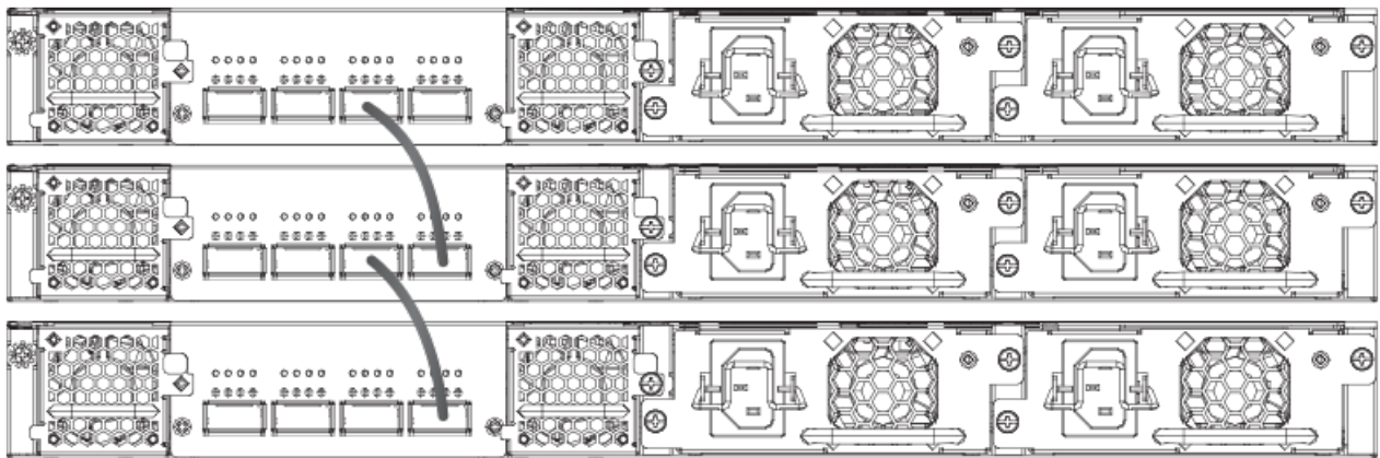
FIGURE 30 ICX 7650 100-Gbps Linear Stack
