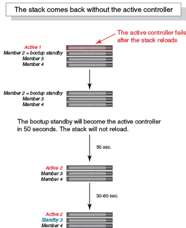
FIGURE 44 Hitless Stacking Failover When the Active Controller Fails
