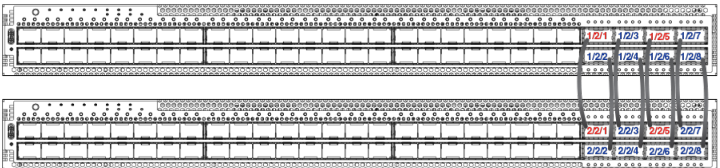
FIGURE 40 ICX 7850-48FS Two-unit Stack with Linear-topology Trunk (Eight Ports)
