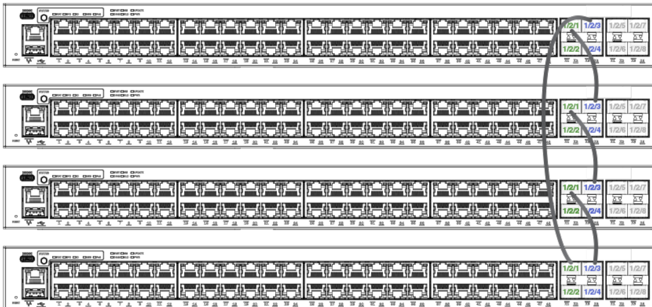
FIGURE 11 ICX 7150-48ZP Stack Ring Topology
